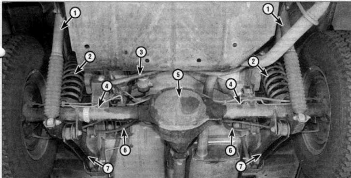
1.2a Rear suspension components (1998 and earlier models)
